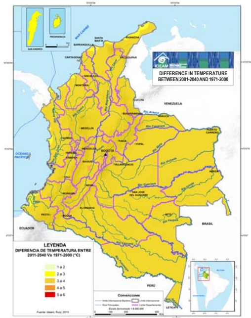
Figure 4.1 Map of the mean temperature difference from the multimodel for the period 2011-2040, compared to 1971-2000.
