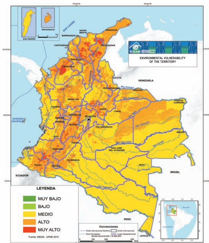
Figure 4.10, Map of environmental vulnerability of the territory, 2011-2040
