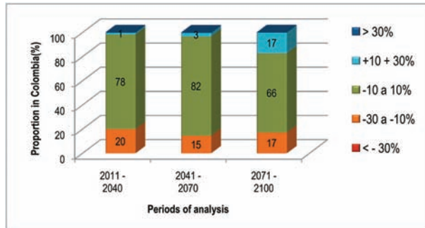
Figure 4.5 Percentage of variation in median annual rainfall (%)
