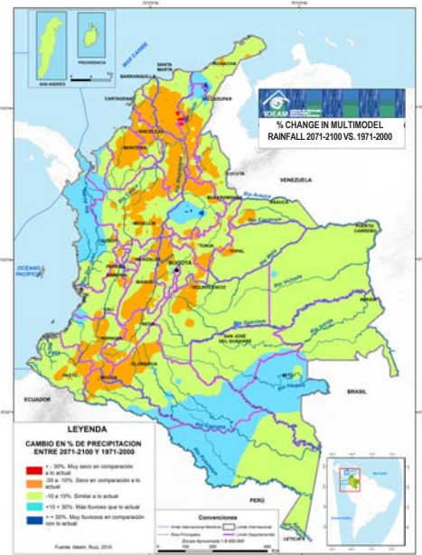
Figure 4.4. (right) Map with percentage change in rainfall for the multimodel for the period 2071-2100 vs 1971-2000.
